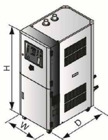
CD-40H ~ 700H
