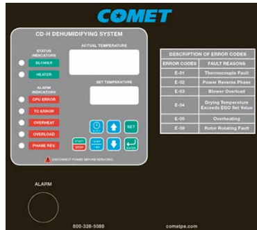
Process Heater Control
