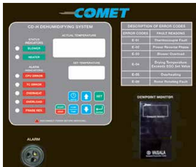
Dewpoint Monitor Installed on the Machine
