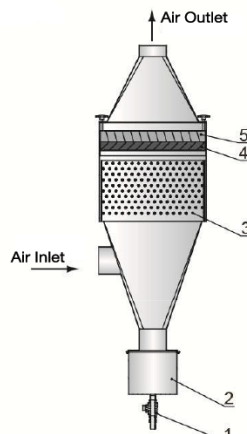
EOF-1000~4000
