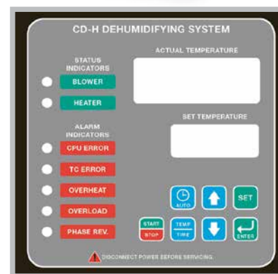
Control Panel
