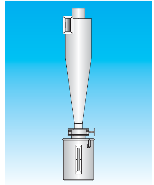
Cyclone Dust Collector ACF
