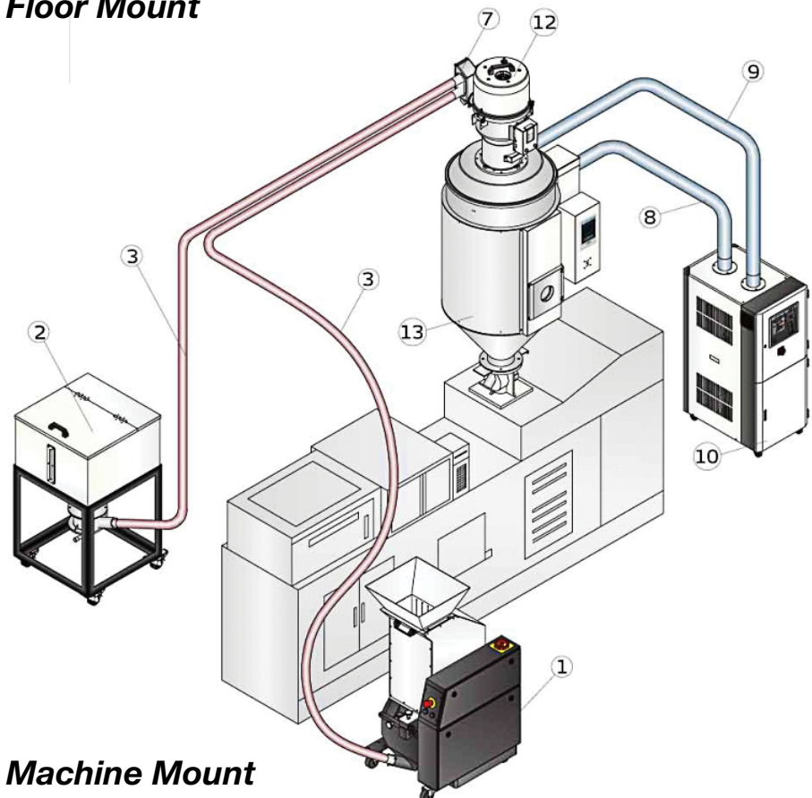
Floor Mount
